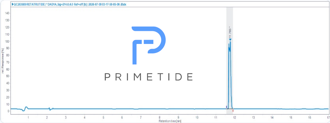
HPLC Chromatogram (Retention Time: 11.769 min)
